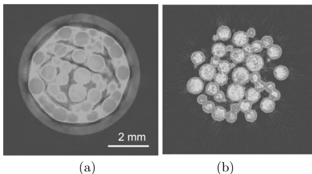
FIG. 5.10. Tomographic slices of spherical sintered copper particles containing beam-hardening artefacts from the X-ray tube used; (a) without correction and (b) with correction (Noethe et al. , 2003).
