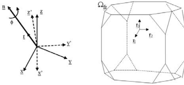
FIG. 9.12. (a): Definition of the Rodrigues vector \mathbf{r} . The co-ordinate system (x, y, z) is rotated around \mathbf{n} by angle \phi into (x', y', z') . \mathbf{r} is parallel to \mathbf{n} : \mathbf{r} = \mathbf{n} \tan(\phi/2) . (b): The fundamental zone in Rodrigues space for face-centred cubic systems
