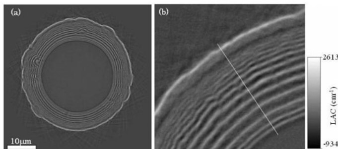
FIG. 7.14. Tomography image of test sample. Concentric multilayer structure is used as a resolution test object for imaging tomography. The outermost structure is 0.15\ \mu\text{m} copper and 0.15\ \mu\text{m} aluminium synthetic multilayer.
