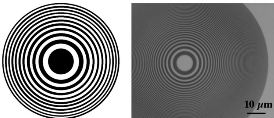
FIG. 7.2. Fresnel zone plate, schematic drawing and optical micrograph. The FZP shown in the optical micrograph has a diameter of 100\text{ }\mu\text{m} and a width of the outermost zone of 250\text{ nm} . This FZP was fabricated by electron beam lithography and is used at the SPring-8 synchrotron radiation beamlines as an objective lens for the X-ray microscope and X-ray microfocusing device (Suzuki et al. , 2001, Takeuchi et al. , 2002).
