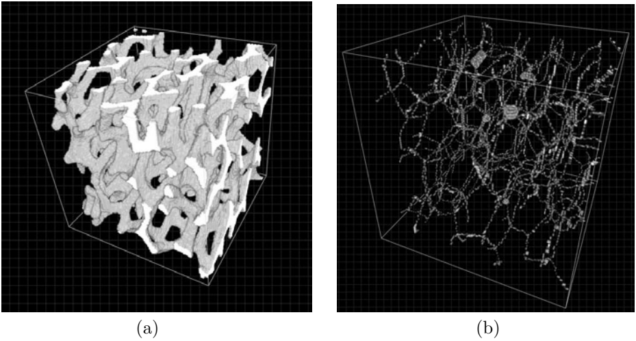
FIG. 3.11. Skeleton for a 128^3 pixel subvolume of the nickel foam from Fig. 3.10. (a) original subvolume, (b) skeleton, skeletonization parameters ( r = \infty, \alpha = \pi ). The skeleton features some small spherical parts. These are the surface of pores within the original strut system. The Euler number for both original and skeleton is -231 .
