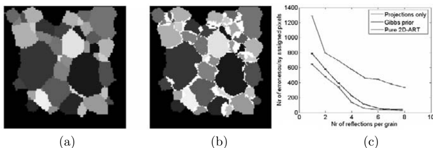
FIG. 9.8. Reconstruction of a 124 \times 124 grain map with 44 undeformed grains. (a) original image. (b) reconstruction using 2D-ART. The white areas indicate areas of ambiguity. (c) Comparison of three reconstruction algorithms: 2D-ART, 2D-ART plus stochastic restorations of ambiguous areas and Grainindex plus stochastic restorations. Shown is the quality of the reconstruction as a function of the number of useful spots per grain. From Alpers et al. (2006) (with permission from the IUC).
