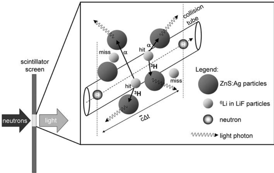
FIG. 13.9. Conversion principle of neutron scintillator screens. A neutron with velocity \bar{c} enters the scintillator and is absorbed by a {}^6\text{Li} nucleus present in the \text{LiF} converter contained in the scintillator. As a result, {}^3\text{H} and {}^4\text{He} reaction products are emitted as positively charged ions that then interact with the \text{ZnS:Ag} particles around in a second step, eventually leading to the emission of visible light that can – at least partially – be detected by conventional imaging systems such as a CCD camera. Some neutrons miss all {}^6\text{Li} nuclei and are not detected. Thus, neutron detection is a two-stage conversion process.
